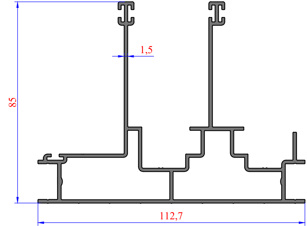
3862 1,936 kg/m
