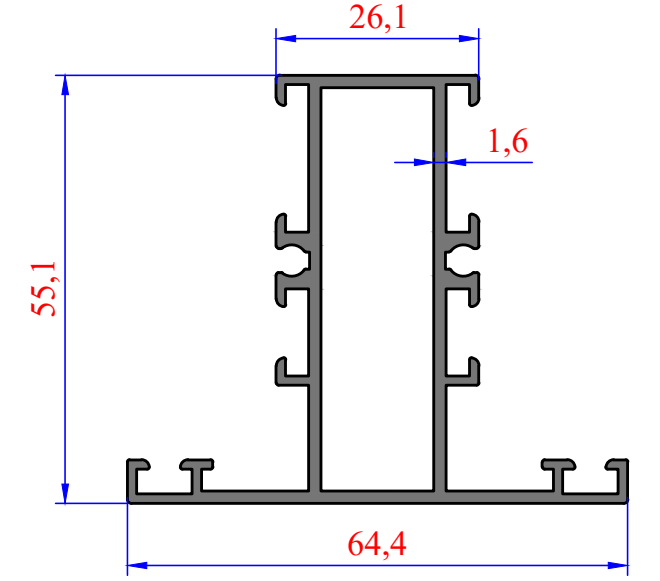
3636 1,070 kg/m SİSTEM 55 DAR ORTA KAYIT
