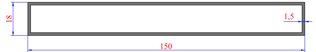
3552 1,343 kg/m
