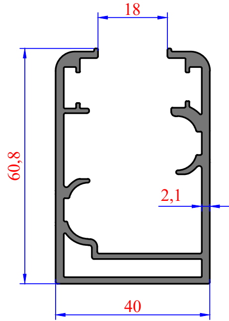
3263 1,294 kg/m Gold Kasa
