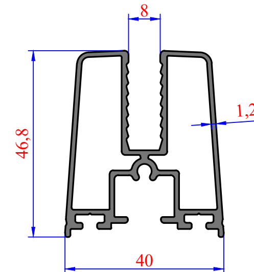
3516 0,940 kg/m Silver Baza
