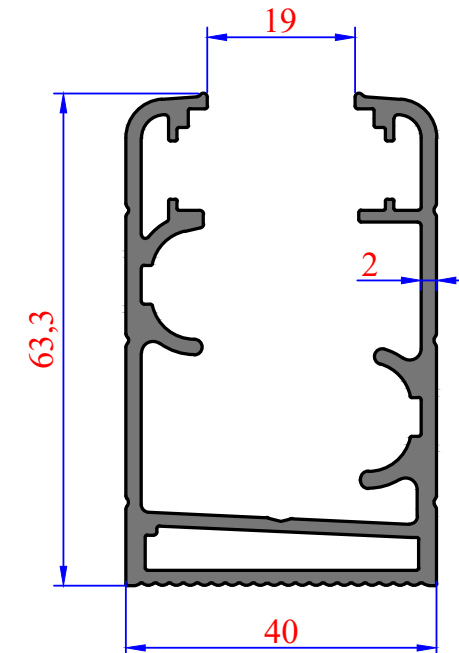
3254 1,428 kg/m Gold Kasa
