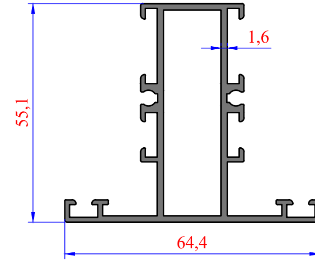
3636 1,070 kg/m SİSTEM 55 DAR ORTA KAYIT
