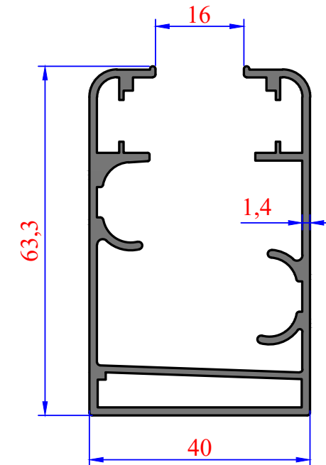
3200 1,094 kg/m Gold Kasa
