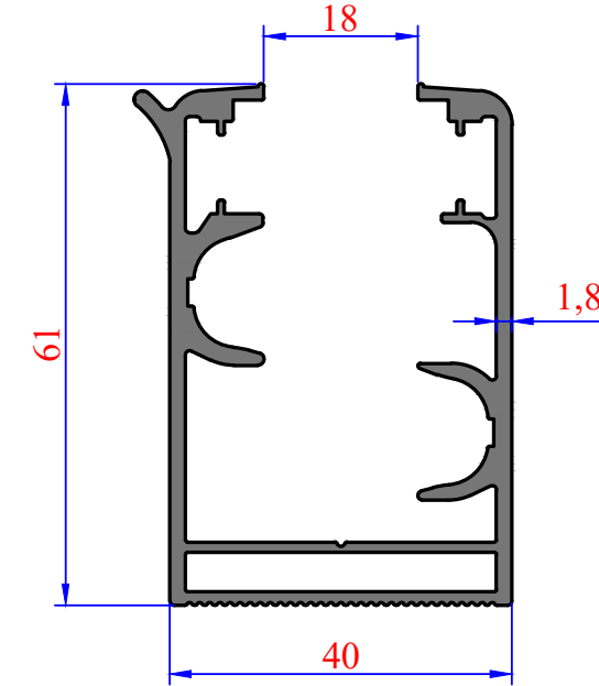
3517 1,291 kg/m Silver Kasa
