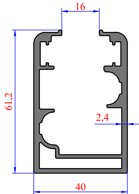
3255 1,504 kg/m Gold Kasa
